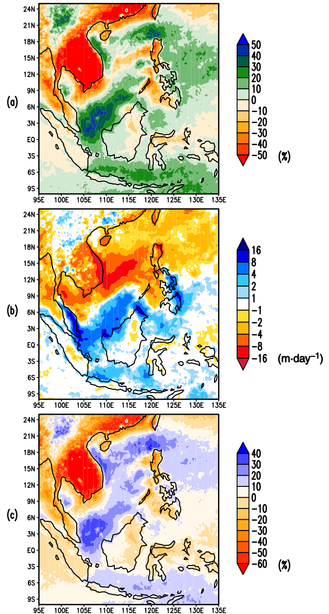
FIGURE 5 Composite difference between (a) cold surge (CS) wet days frequency and seasonal wet days frequency; (b) CS wet days intensity and seasonal wet days intensity; (c) CS extreme rainfall event frequency and seasonal extreme rainfall event frequency. Wet days are defined as days with rainfall \geq 1 \text{ mm} . Extreme rainfall events are defined as days with rainfall exceeding the 95th percentile of seasonal rainfall. The percentage is the percentage difference between CS wet days frequency and seasonal wet day frequency [Colour figure can be viewed at wileyonlinelibrary.com]
